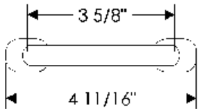
CK310 Sash Cabinet Pull, 3 5/8"
