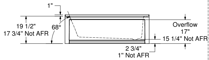
WHIRLPOOL SYSTEM
